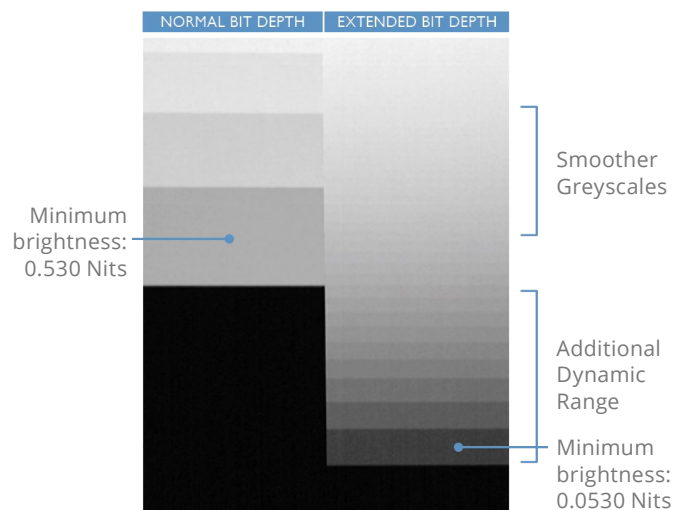
Banded Gradient: "Performance at 0.05% brightness with Dark Magic disabled, illustrating PWM bit depth improvement: Frame grab from camera footage of 2000 Nits panels running at just 1 Nit."
