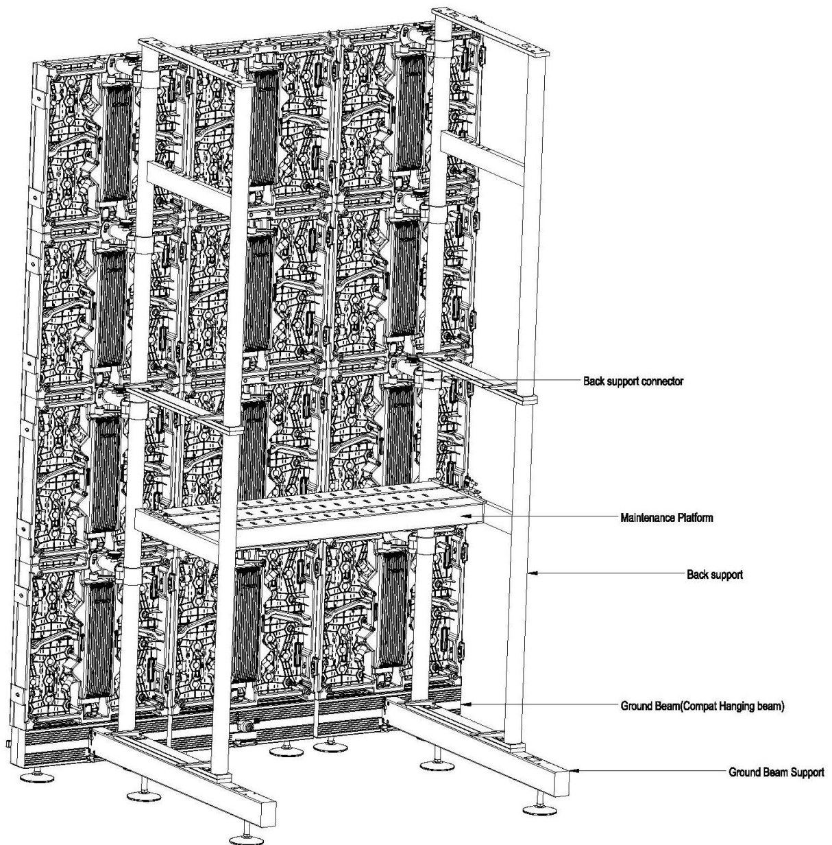
Fig5. Stacking Diagram
