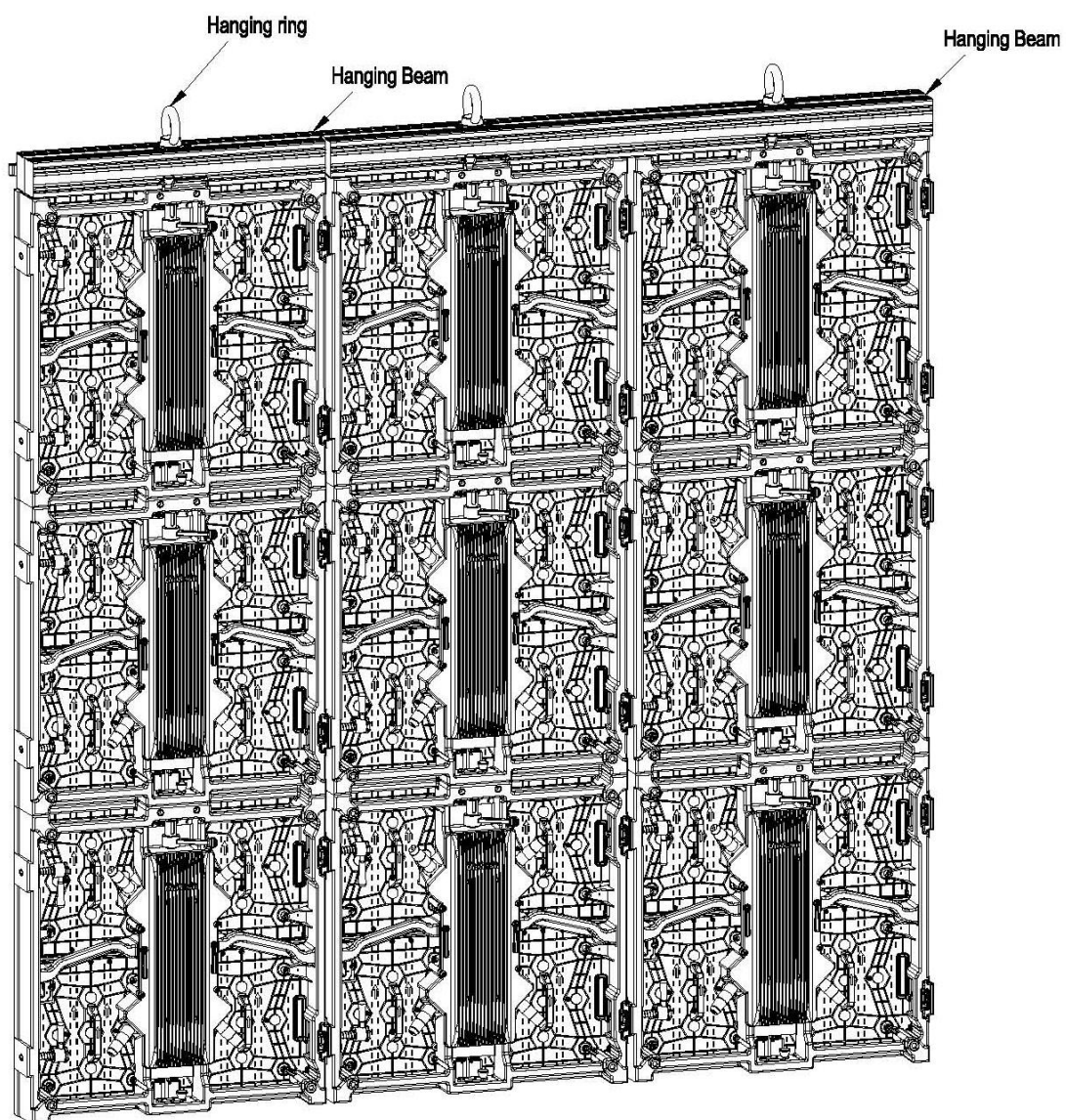
Fig3. Hanging Diagram
