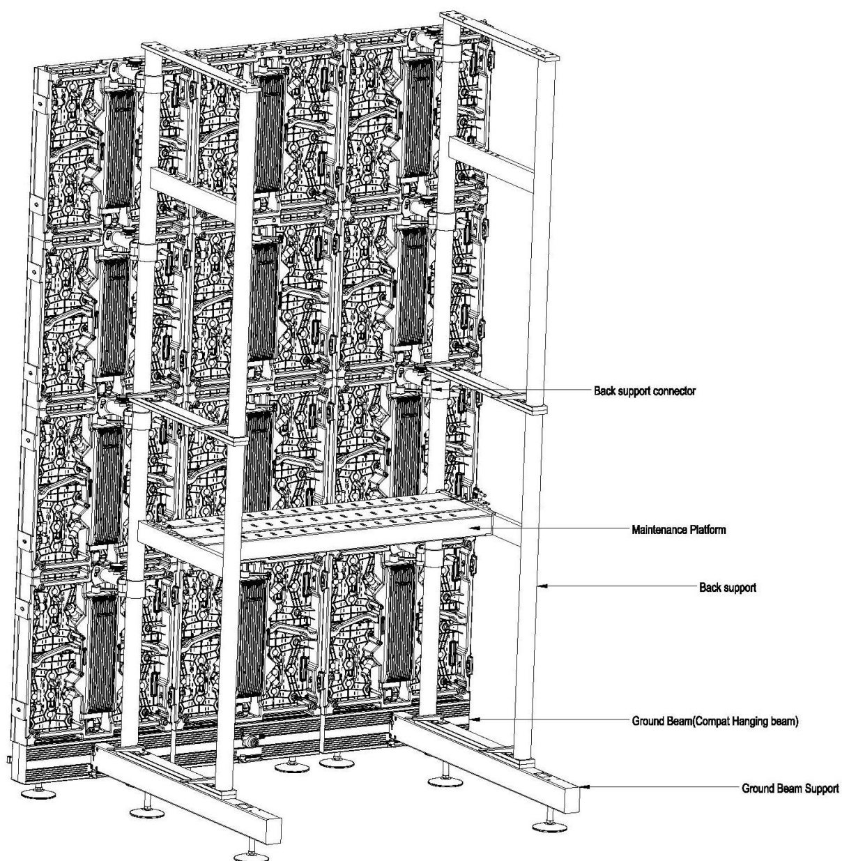
Fig5. Stacking Diagram
