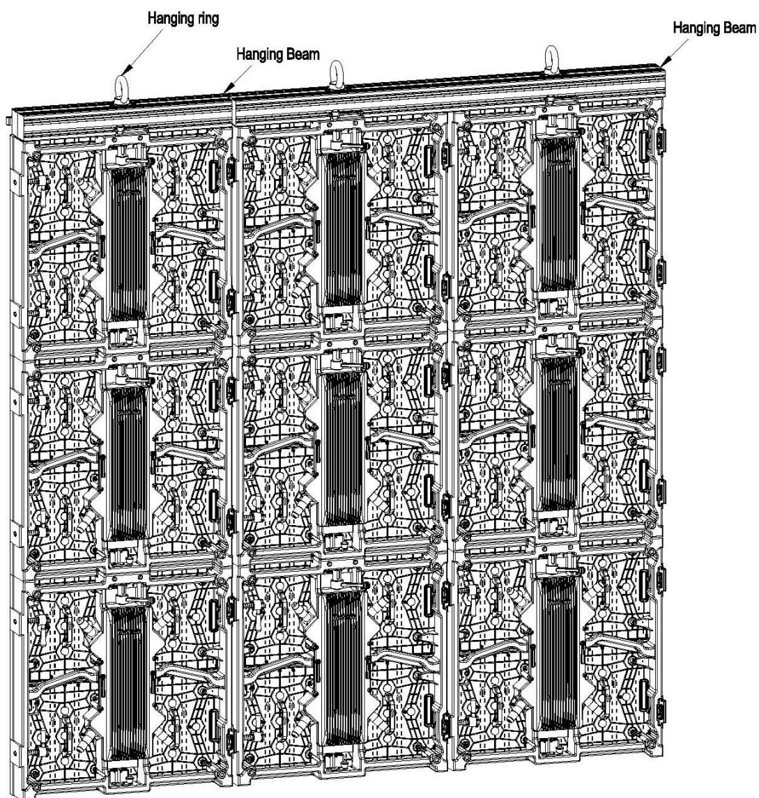
Fig3. Hanging Diagram
